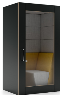
SES 11-G 1-seater booth Flat roof Upholstered panels 1100W x 750D x 2000H mm
