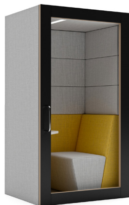
SES 11-UG 1-seater booth Flat roof Upholstered panels 1100W x 750D x 2000H mm
